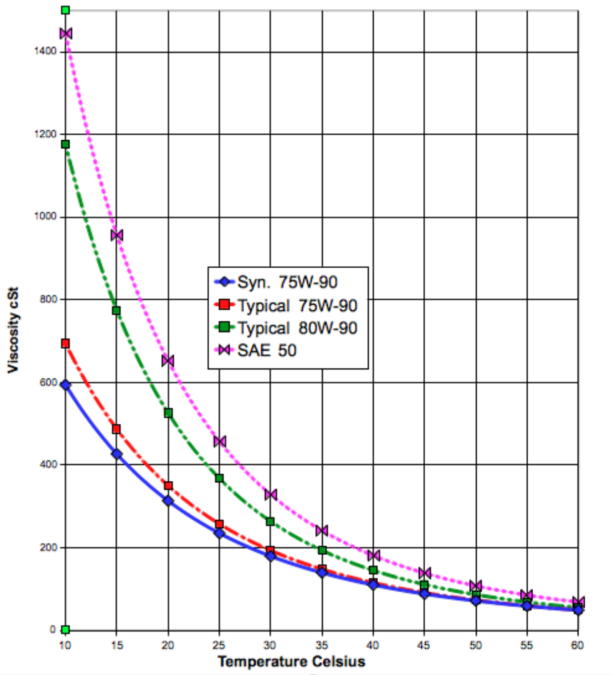
Viscosity Curve
